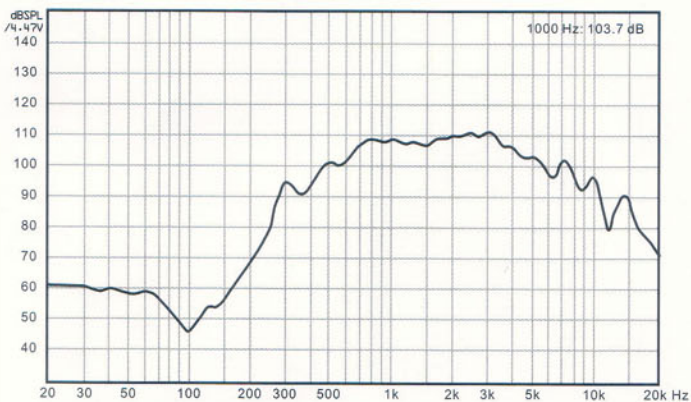
Frequency Response
